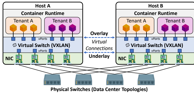
Figure 1: Architectural overview of our in-production multi-tenant large model training infrastructure built on top of the RDMA NIC- and VXLAN-based container network.
